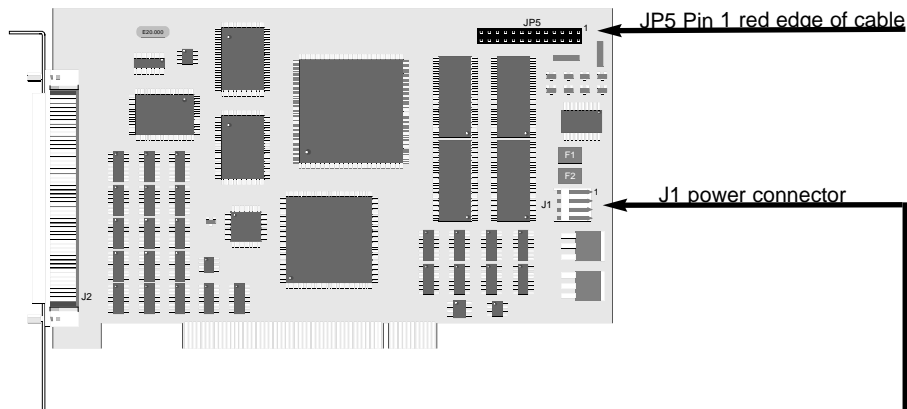
Figure 1: PXD1000 showing JP5 and J1
